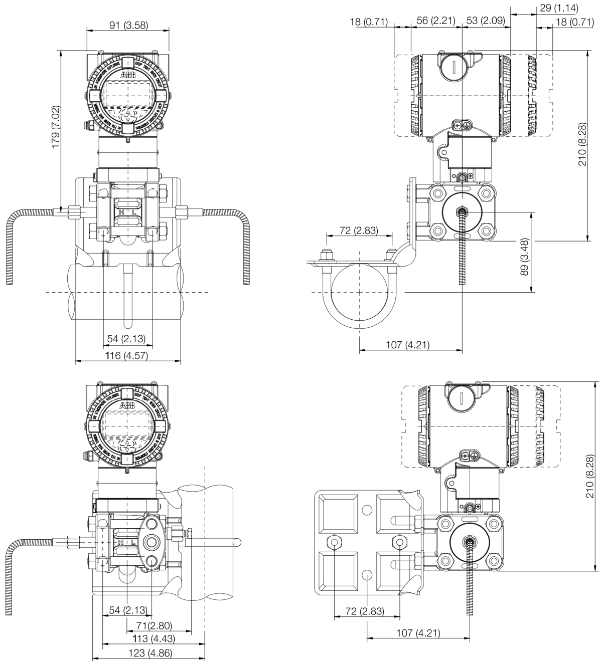
Fig. 6: Pipe mounting - Barrel housing
