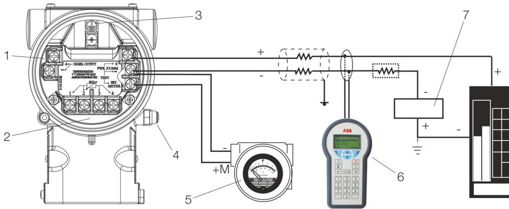
Fig. 9: Electrical connections
