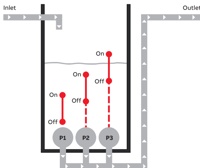
Figure 10 Independent on and off trip points
