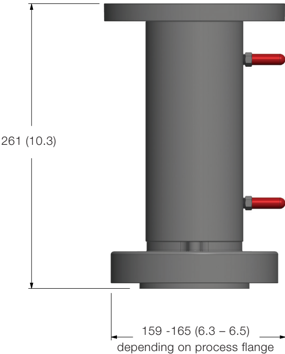
Cooling tube with high pressure flange
